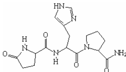
Figure 4-1. TRH molecule.
